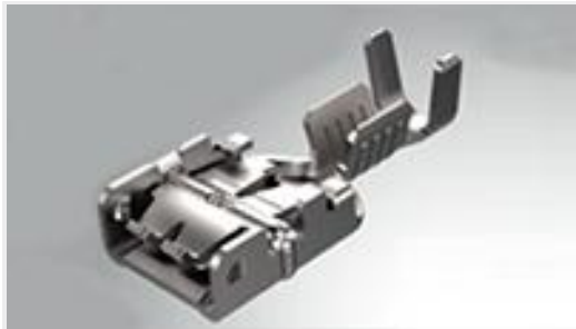
TE Part #336075-3 250 FASTON,REC.,20-16 AWG,PTBR
