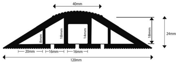
Snapfit Type MCP/2
