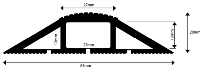
Snapfit Type MCP/1
