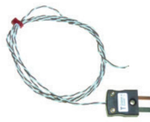
Type T PTFE Exposed Junction with Miniature Plug
