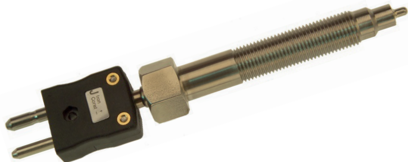
A 1/2"UNF-20 Melt Bolt Thermocouple with Type 'J' Thermocouple Plug
