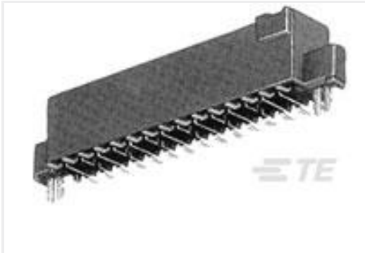
TE Part #5-147384-2 20 50/50 GRID SMT RCPT VC LF
