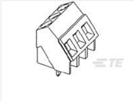
TE Part #796689-3 TERMI-BLOK PCB MOUNT 3P.
