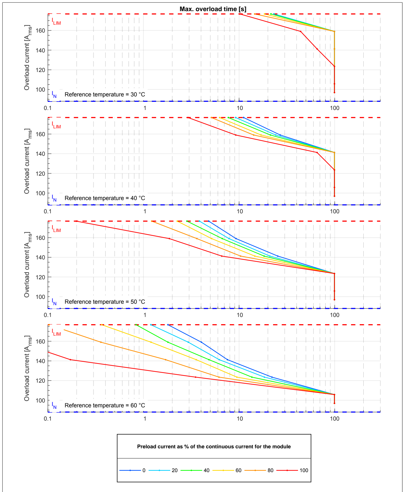
Figure 2: 8BVI0880HCSx.008-x - Overload characteristics, overload response - ERROR+STOP
