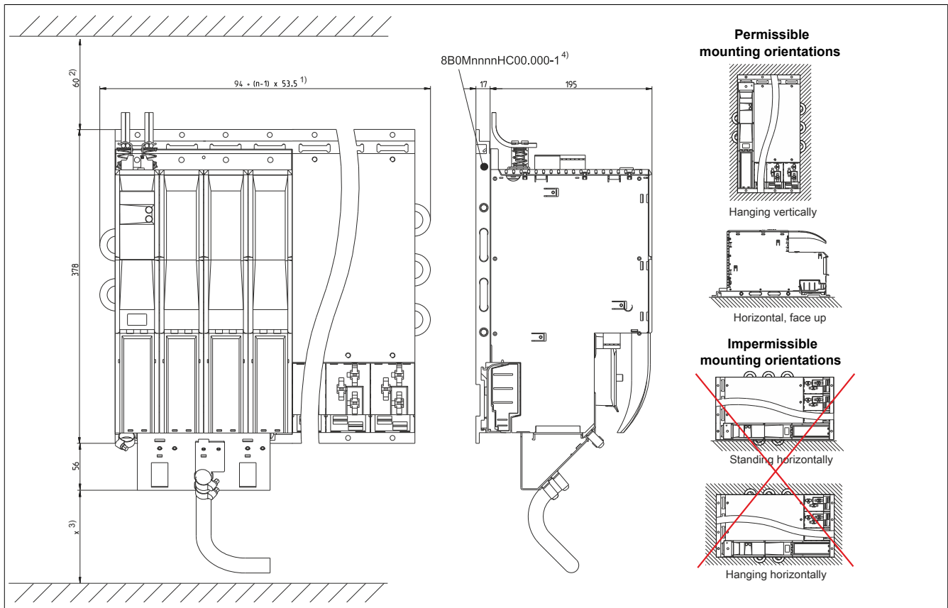
Figure 6: Cold plate - Dimension diagram and installation dimensions
