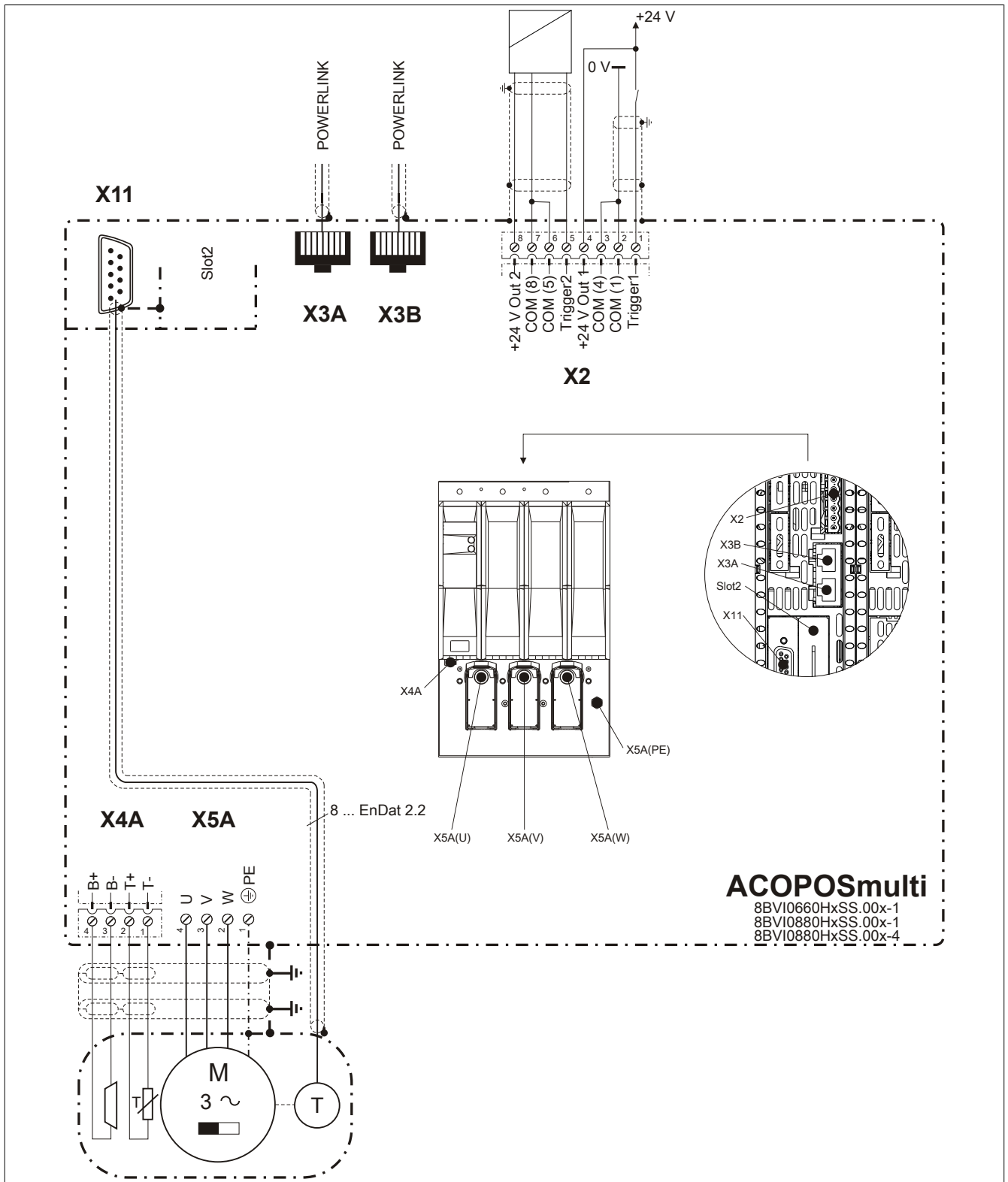
Figure 8: Pinout overview
