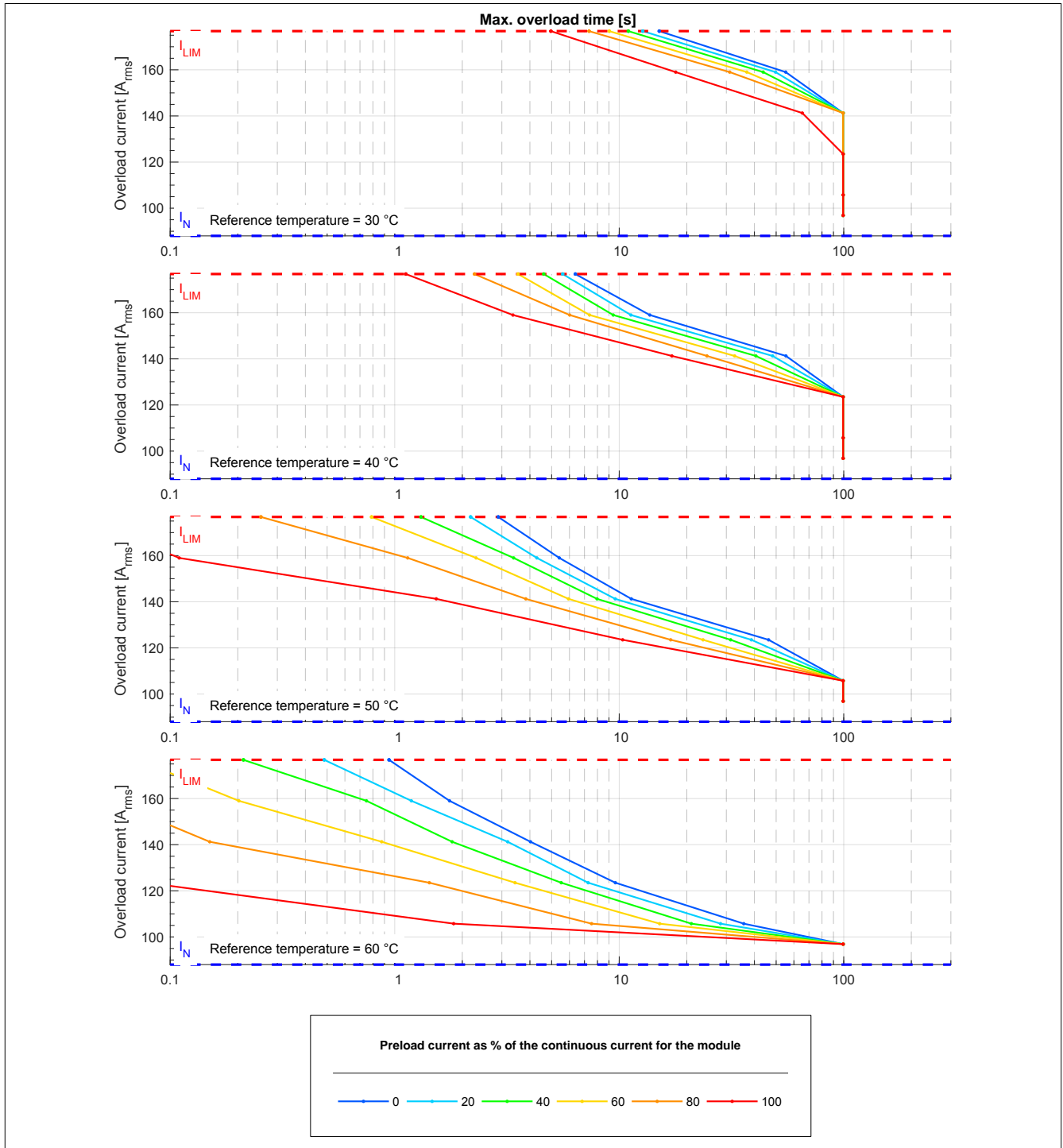
Figure 1: 8BVI0880HCSx.008-x - Overload characteristics, overload response - WARNING
