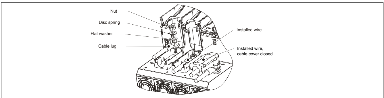
Figure 9: X5A - Cable installation
