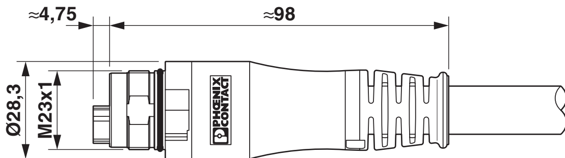
Dimensional drawing
