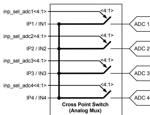
Figure 10: ADC input signals through Cross Point Switch
