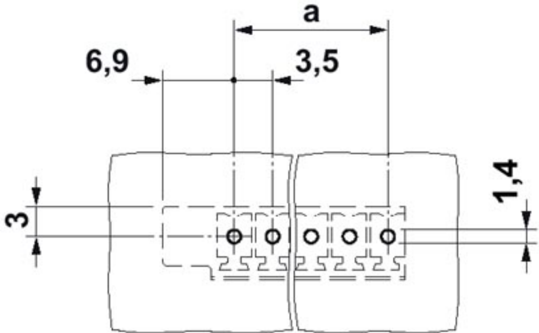
Drilling diagram
