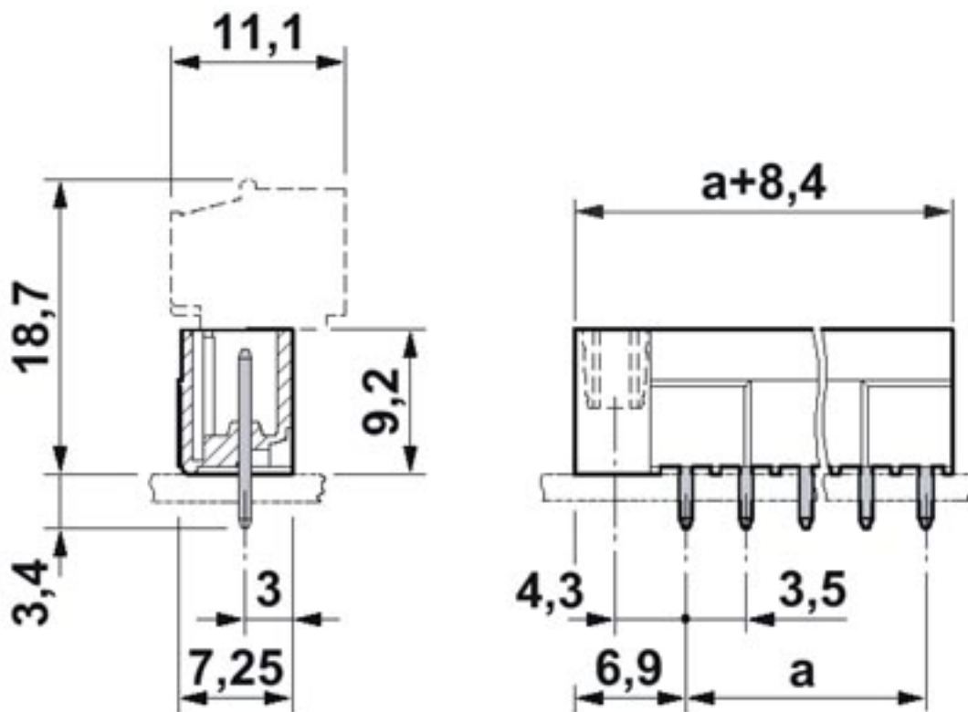
Dimensioned drawing
