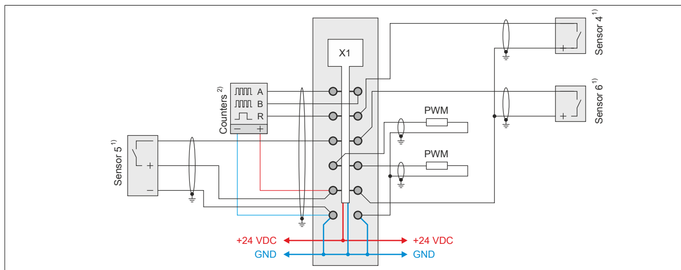
Figure 3: Connection example 2 (X1)
