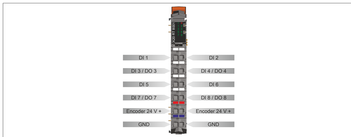
Figure 1: Pinout (X1)
