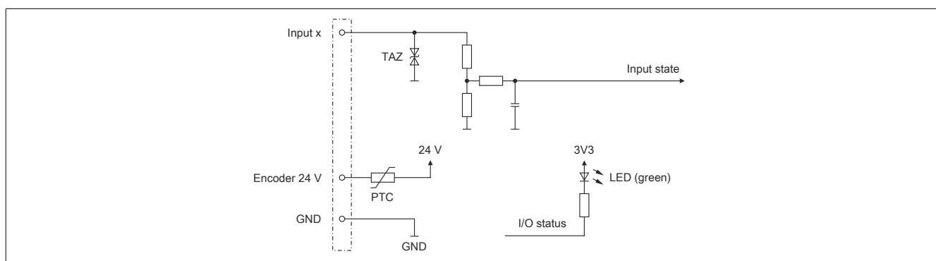
Figure 4: Input circuit diagram of digital inputs (X1)
