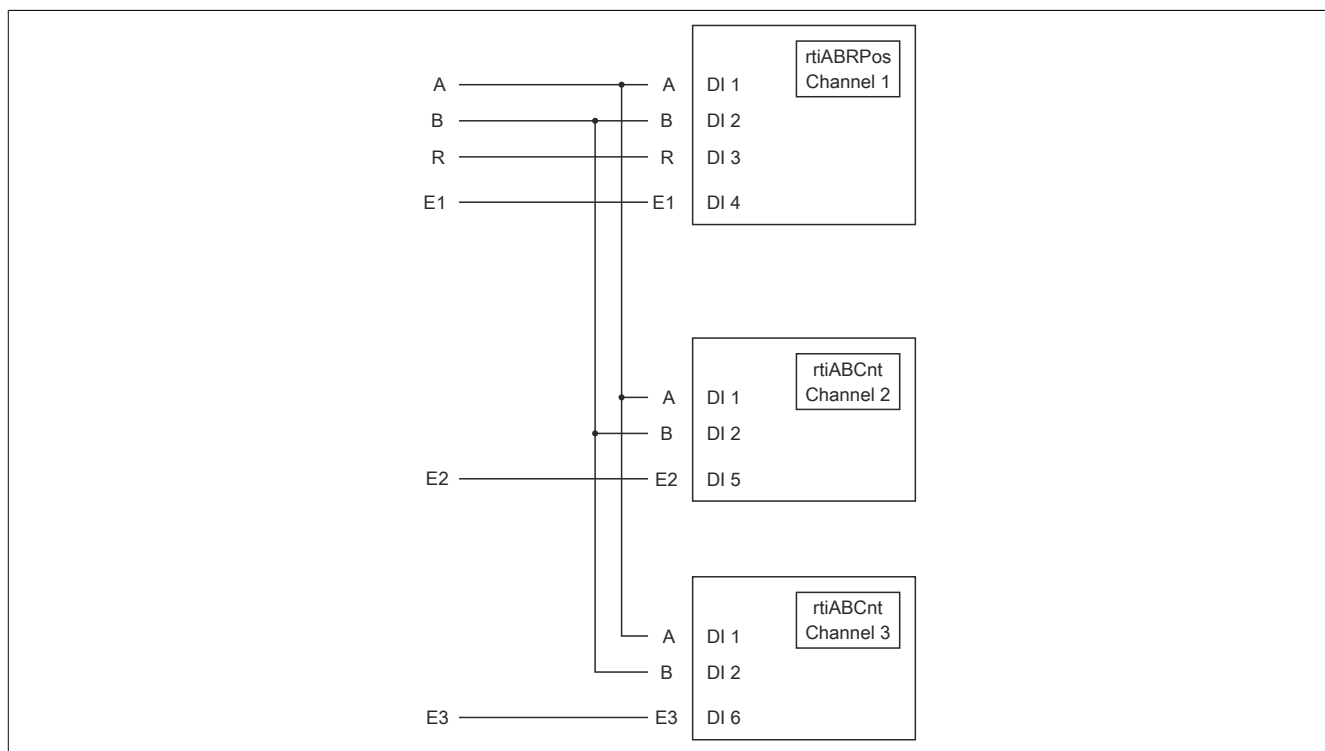
Figure 8: Diagram of input signals when using rtiABRPos and rtiABCnt at the same time
