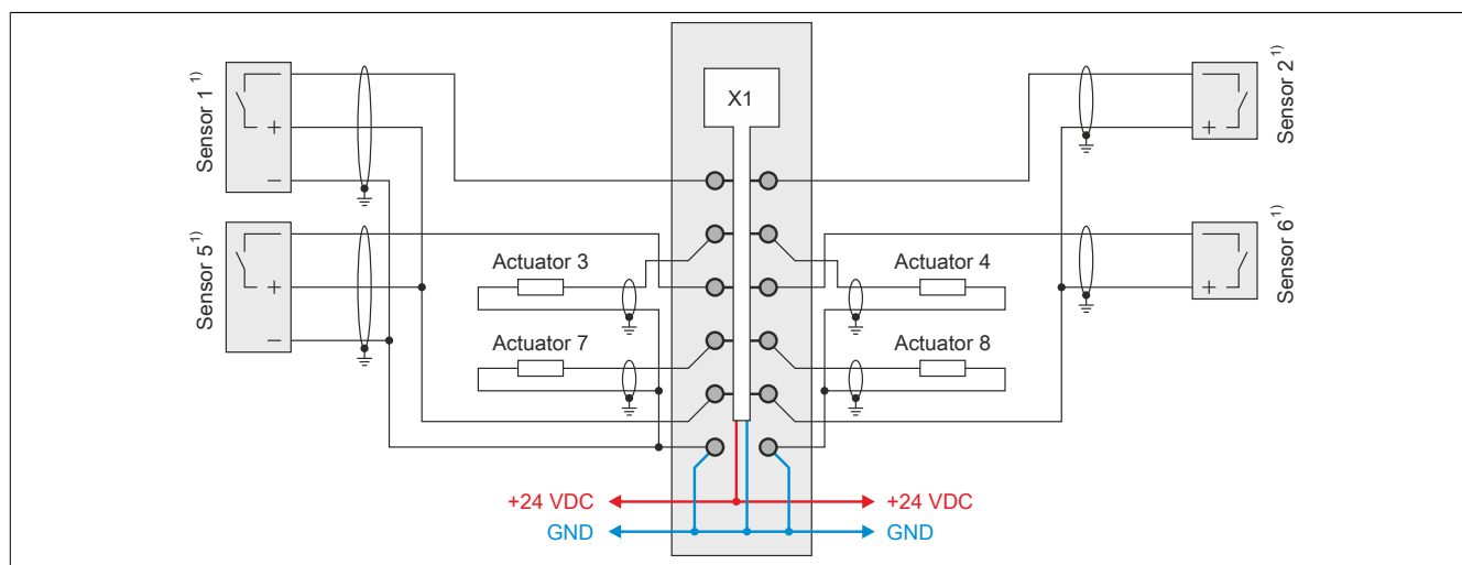
Figure 2: Connection example 1 (X1)
