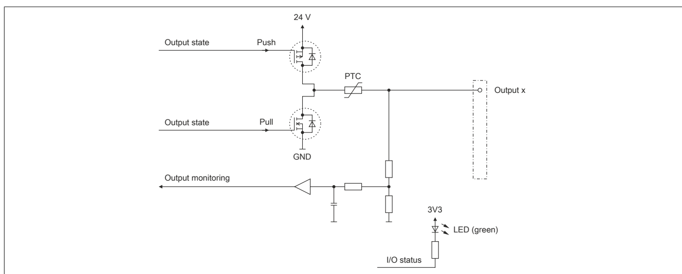
Figure 5: Input/Output circuit diagram of digital mixed channels (X1)
