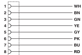
Contact assignment of M8 socket
