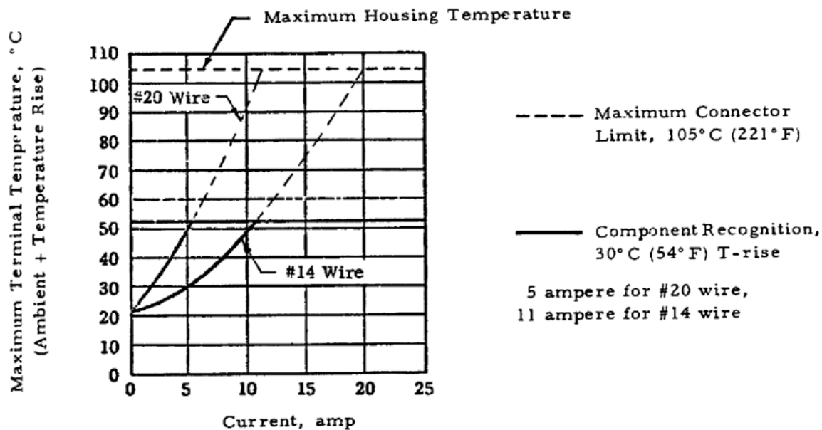
Terminal Temperature vs Current/Circuit, Phosphor Bronze Contacts, 4 Circuit Free Hanging Housing
