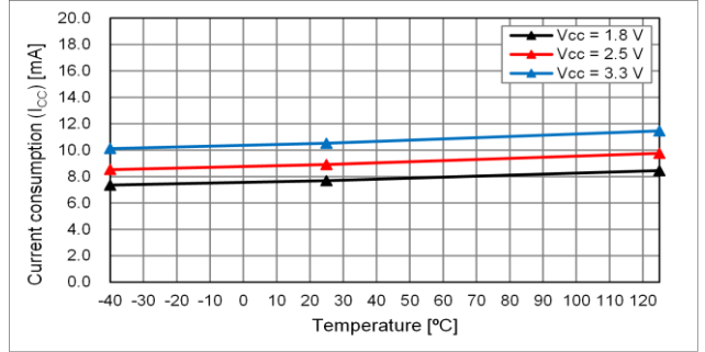
fo = 125 MHz
