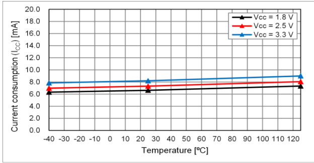
fo = 76.8 MHz
