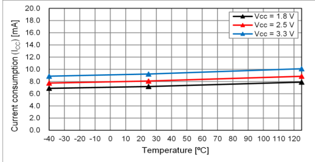
fo = 100 MHz
