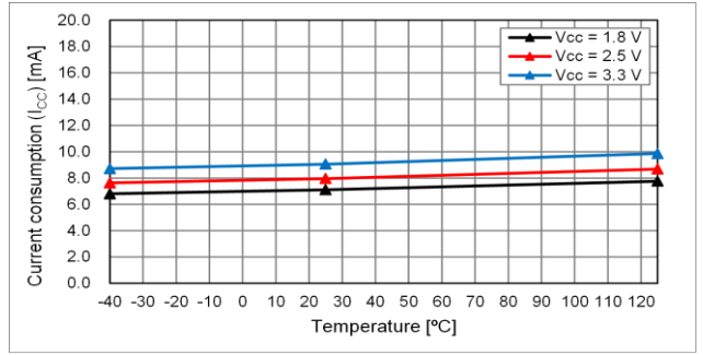
fo = 98.304 MHz
