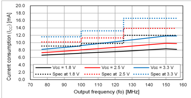
No load
