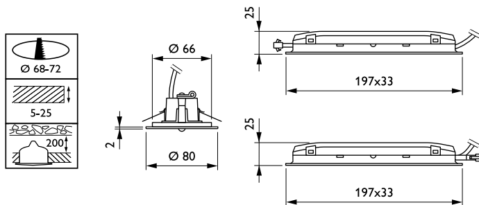
Emergency downlight EM120B
