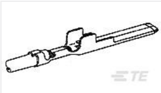
TE Part #170221-3 TAB WITH LANCE FOR M.I.C.
