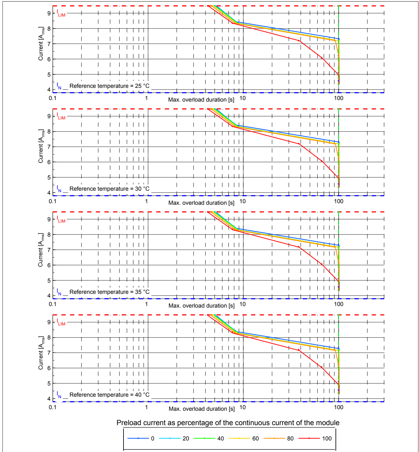
Figure 1: 8BVI0028HWDx.000-x - Overload characteristics, overload response - WARNING
