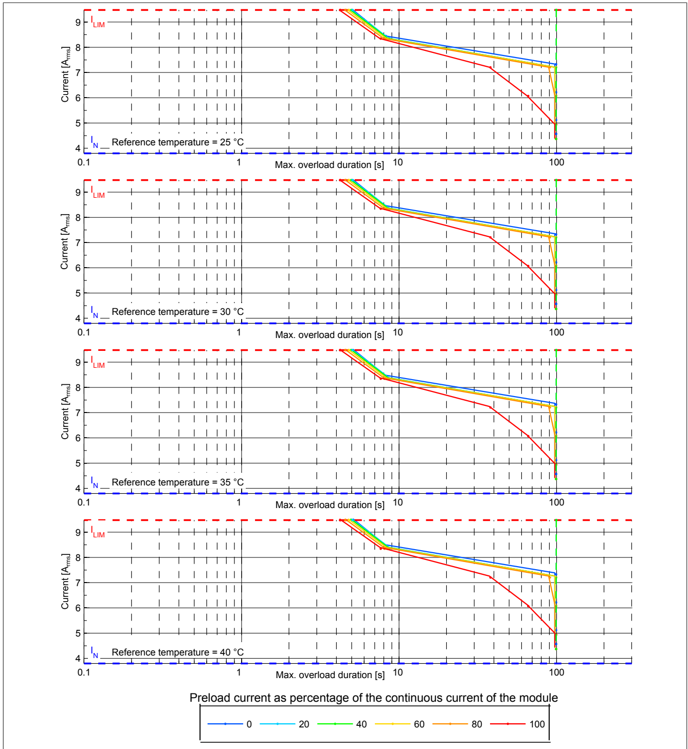
Figure 2: 8BVI0028HWDx.000-x - Overload characteristics, overload response - ERROR + STOP
