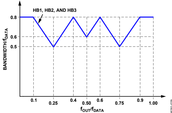
Figure 59. Signal Bandwidth vs. Center Frequency of the Output Signal, 8\times Interpolation
