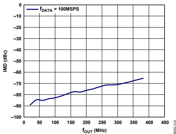
Figure 18. IMD vs. f_{OUT} , 8 \times Interpolation, f_{DATA} = 100 MSPS, Digital Scale = 0 dBFS, I_{FS} = 20 mA
