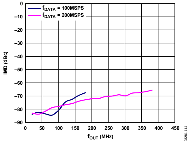
Figure 17. IMD vs. f_{OUT} over f_{DATA} , 4 \times Interpolation, Digital Scale = 0 dBFS, I_{FS} = 20 mA
