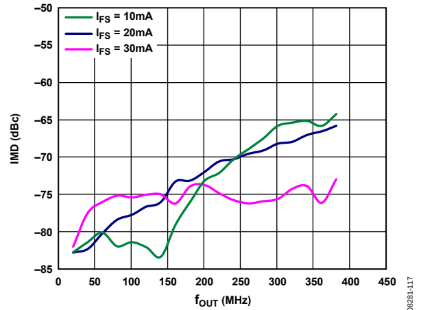
Figure 20. IMD vs. f_{OUT} over I_{FS} , 2 \times Interpolation, f_{DATA} = 400 MSPS, Digital Scale = 0 dBFS
