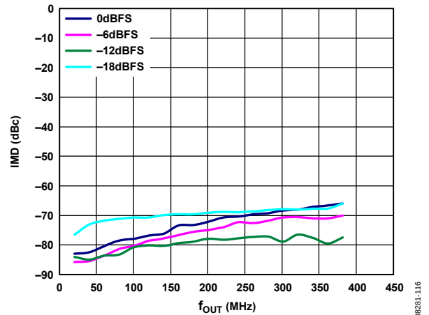
Figure 19. IMD vs. f_{OUT} over Digital Scale, 2 \times Interpolation, f_{DATA} = 400 MSPS, I_{FS} = 20 mA
