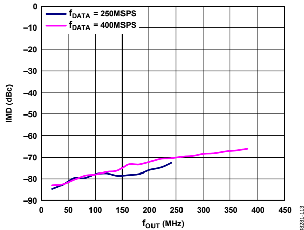
Figure 16. IMD vs. f_{OUT} over f_{DATA} , 2 \times Interpolation, Digital Scale = 0 dBFS, I_{FS} = 20 mA
