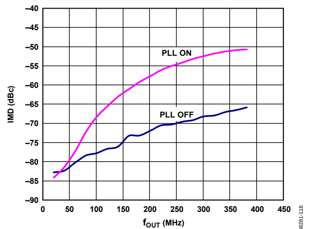
Figure 21. IMD vs. f_{OUT} , 4 \times Interpolation, f_{DATA} = 200 MSPS, Digital Scale = 0 dBFS, I_{FS} = 20 mA, PLL On and PLL Off
