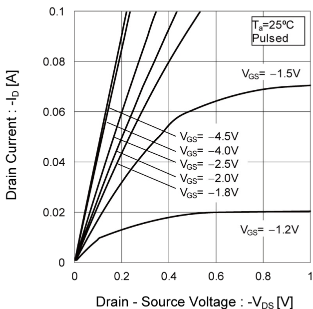
Fig.22 Typical Output Characteristics(I)
