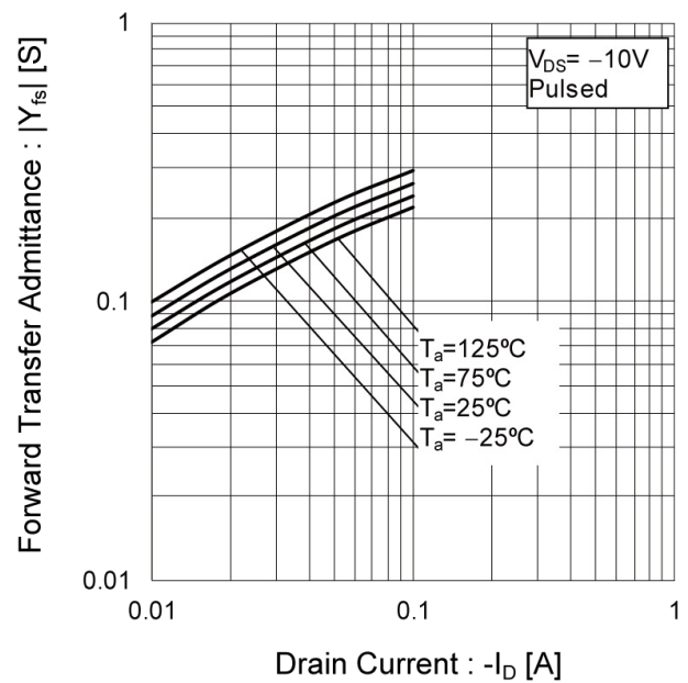
Fig.27 Forward Transfer Admittance vs. Drain Current
