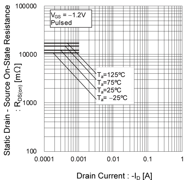
Fig.35 Static Drain - Source On - State Resistance vs. Drain Current (VI)
