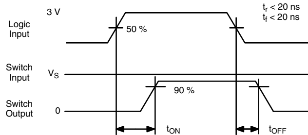
Figure 2. Switching Time
