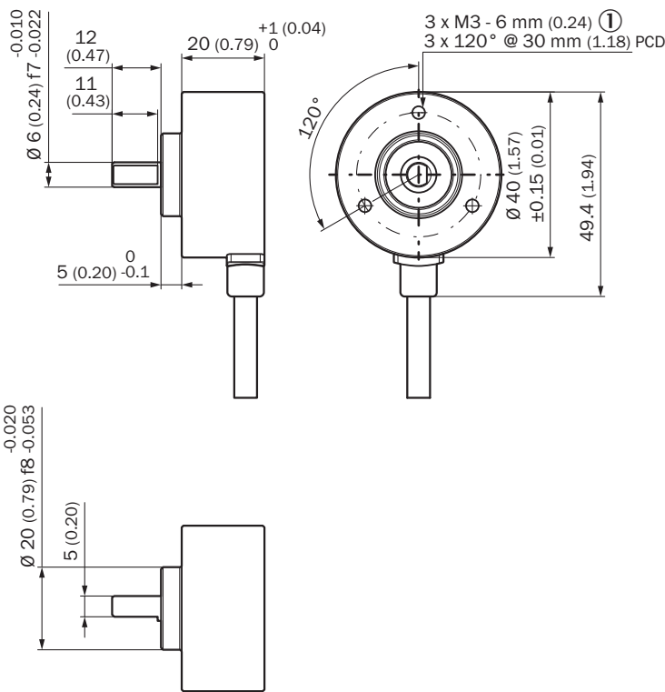
Dimensions in mm (inch) ① depth
