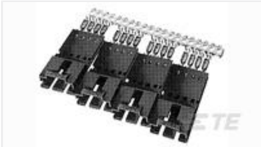
TE Part #103946-4 4X5 MTE SHRD PIN SR POL .100CL
