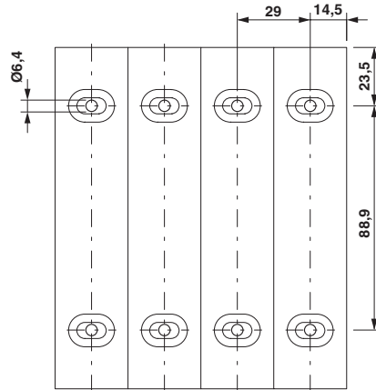
Dimensional drawing
