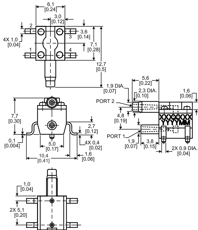
Figure 3. Mounting Dimensions (continued)
