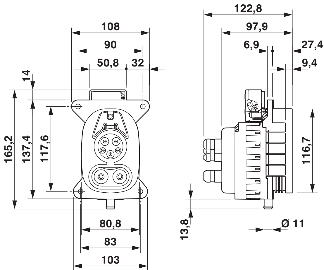
Dimensional drawing
