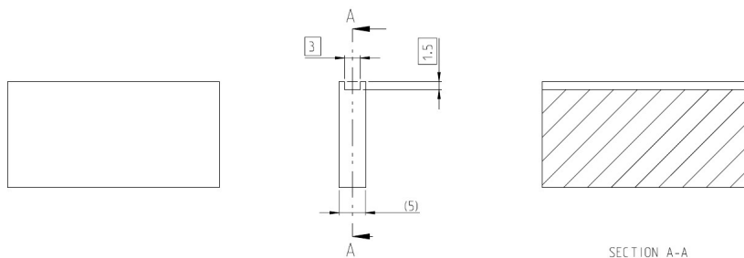
Recommended Panel_bottom dimension 推荐下面板尺寸
