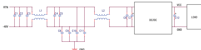
Figure 5. Conducted Emissions Test Circuit
