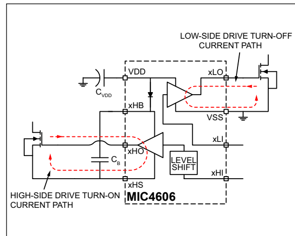
FIGURE 7-13: Turn-Off Current Paths.
