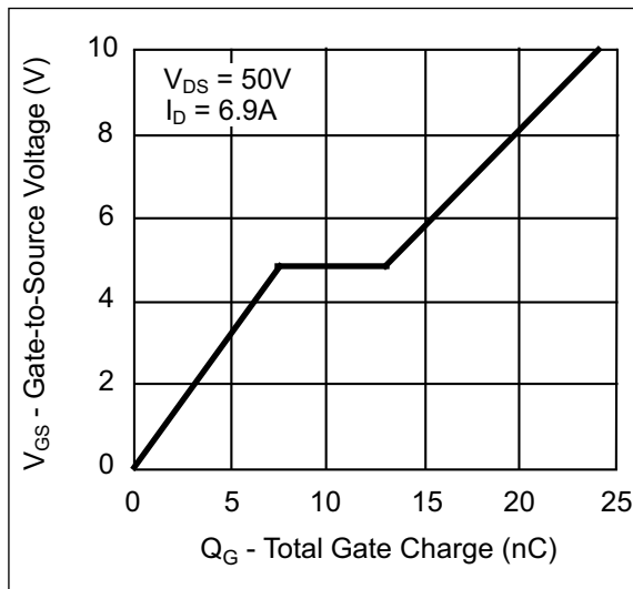
FIGURE 7-8: Typical Gate Charge vs. V_{GS} .
