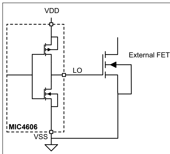
FIGURE 6-1: Low-Side Driver Block Diagram.
