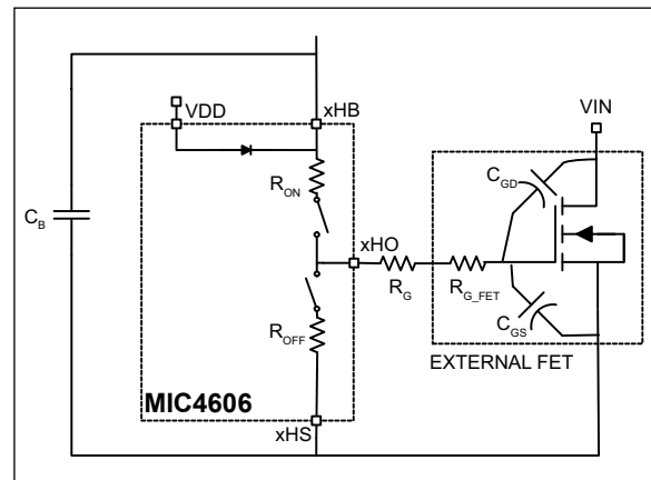
FIGURE 7-7: MIC4606 Driving an External High-Side MOSFET.
