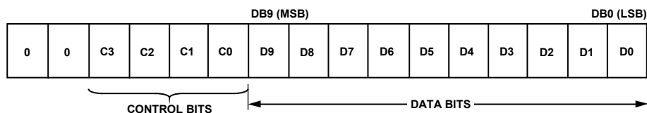
Figure 2. Shift Register Contents
