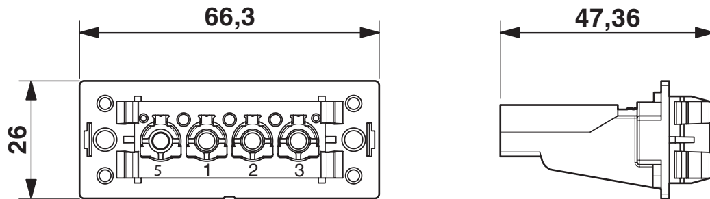
Dimensional drawing
