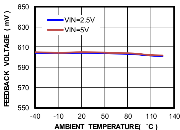
Feedback Voltage vs. T_A
