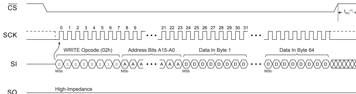
Figure 8-2. Page Write
