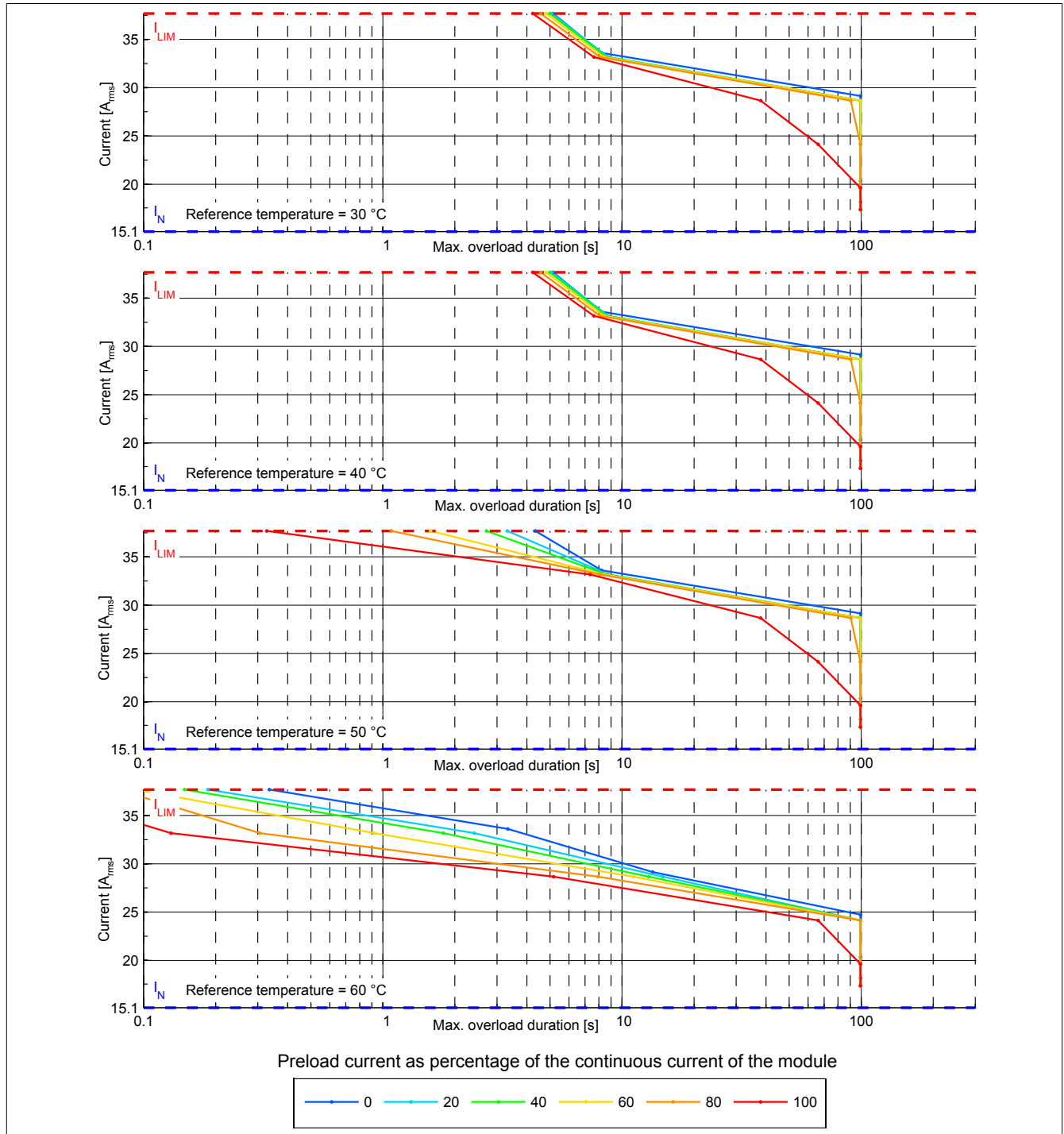
Figure 1: 8BVI0110HCSS.000-x - Overload characteristics, overload response - WARNING
