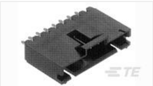
TE Part #1-103670-0 11 MTE HDR SRST LATCH W/HLDWN
