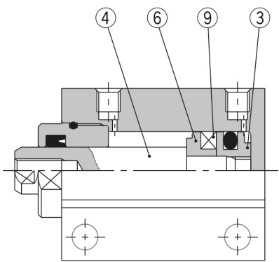
Built-in magnet
