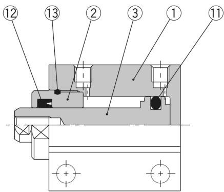
Without magnet
