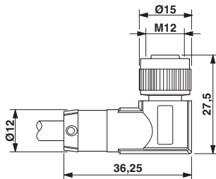
Socket M12-SPEEDCON, angled, shielded
