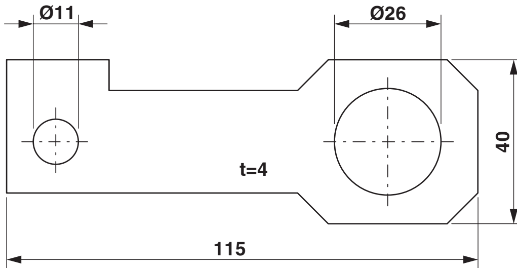
Dimensional drawing
