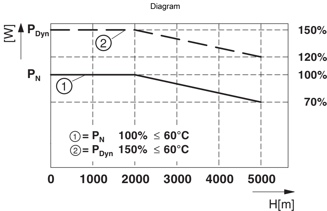
Altitude-dependent derating
