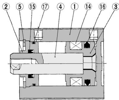
Rod end male thread
