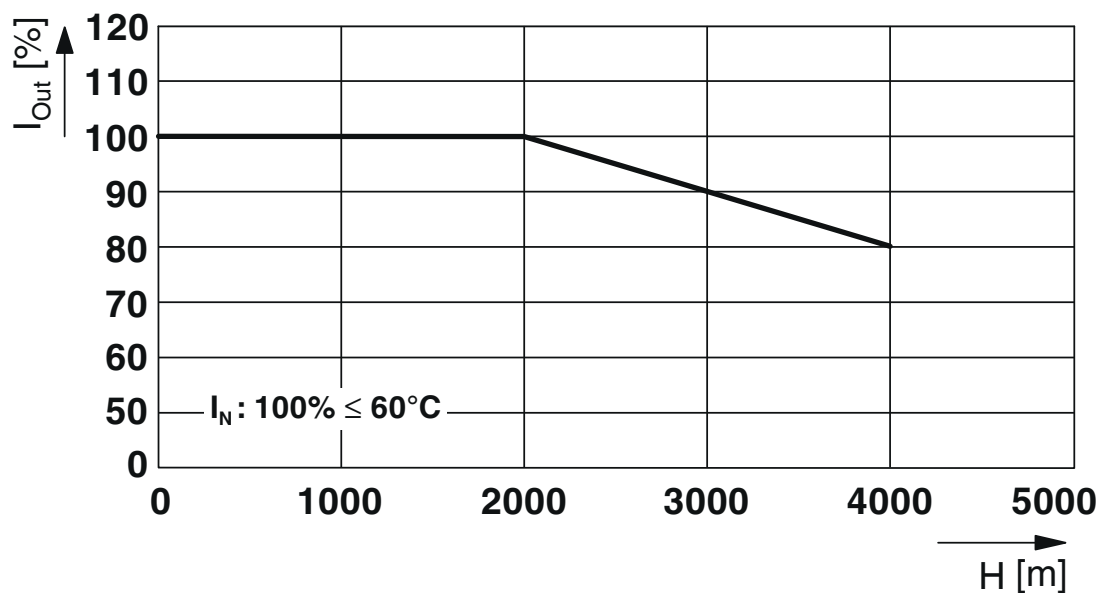
Output current/installation altitude
