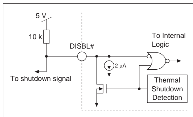
Figure 6.1 THDN Signal to the System Controller
