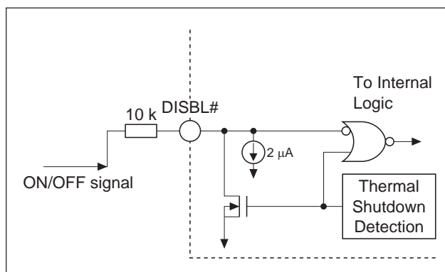
Figure 6.2 ON/OFF Signal from the System Controller
