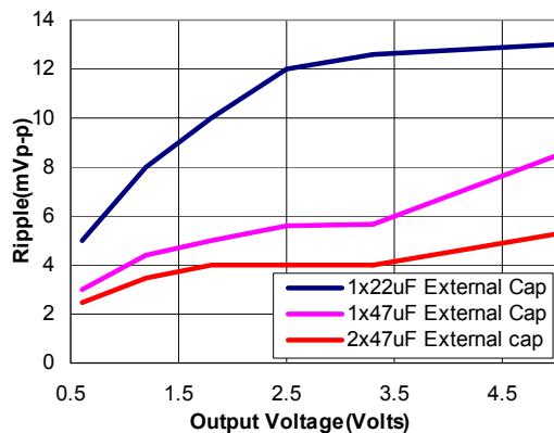
Figure 52. Output ripple voltage for various output voltages with external 1x22 \mu\text{F} , 1x47 \mu\text{F} or 2x47 \mu\text{F} ceramic capacitors at the output (2A load). Input voltage is 12V.
