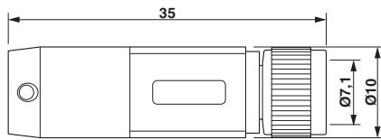
Dimensioned drawing
