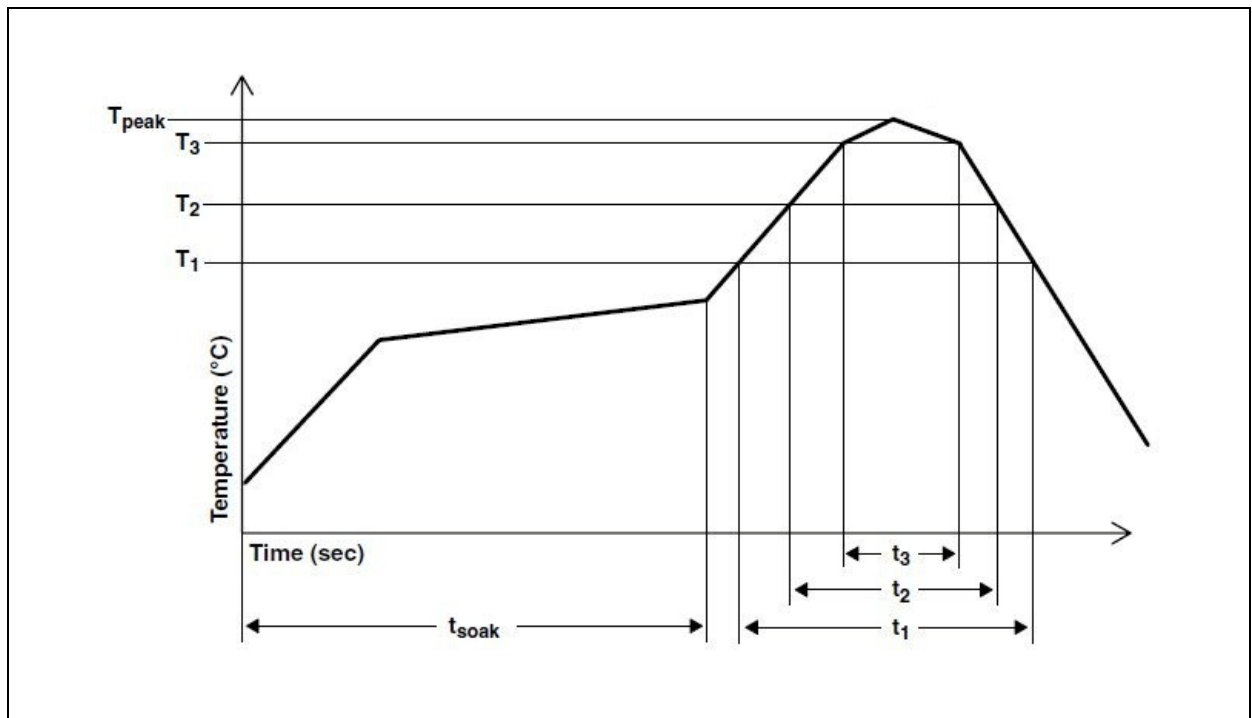
Figure 21: Solder Reflow Profile Graph
