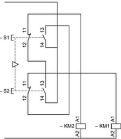
Control of Single-Speed Reversing Motor With ZBE2BE101 + ZB2BE102
