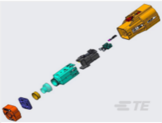
TE Part #YHVA630-2PHM-4MM-A HVA630-2phm,4sqmm,Key A
