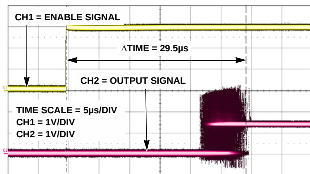
FIGURE 18. ENABLE TIME (WORST CASE)
