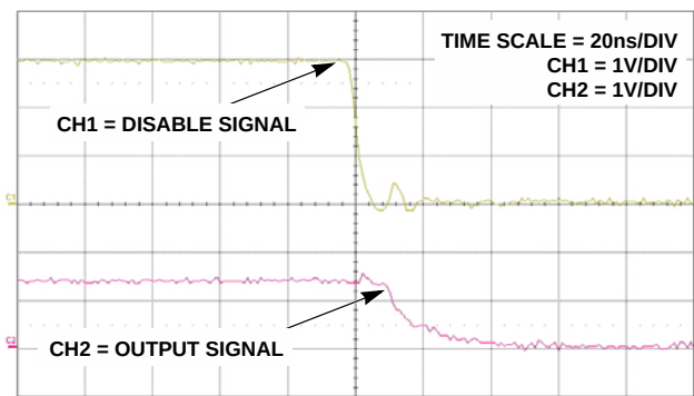
FIGURE 17. DISABLE TIME
