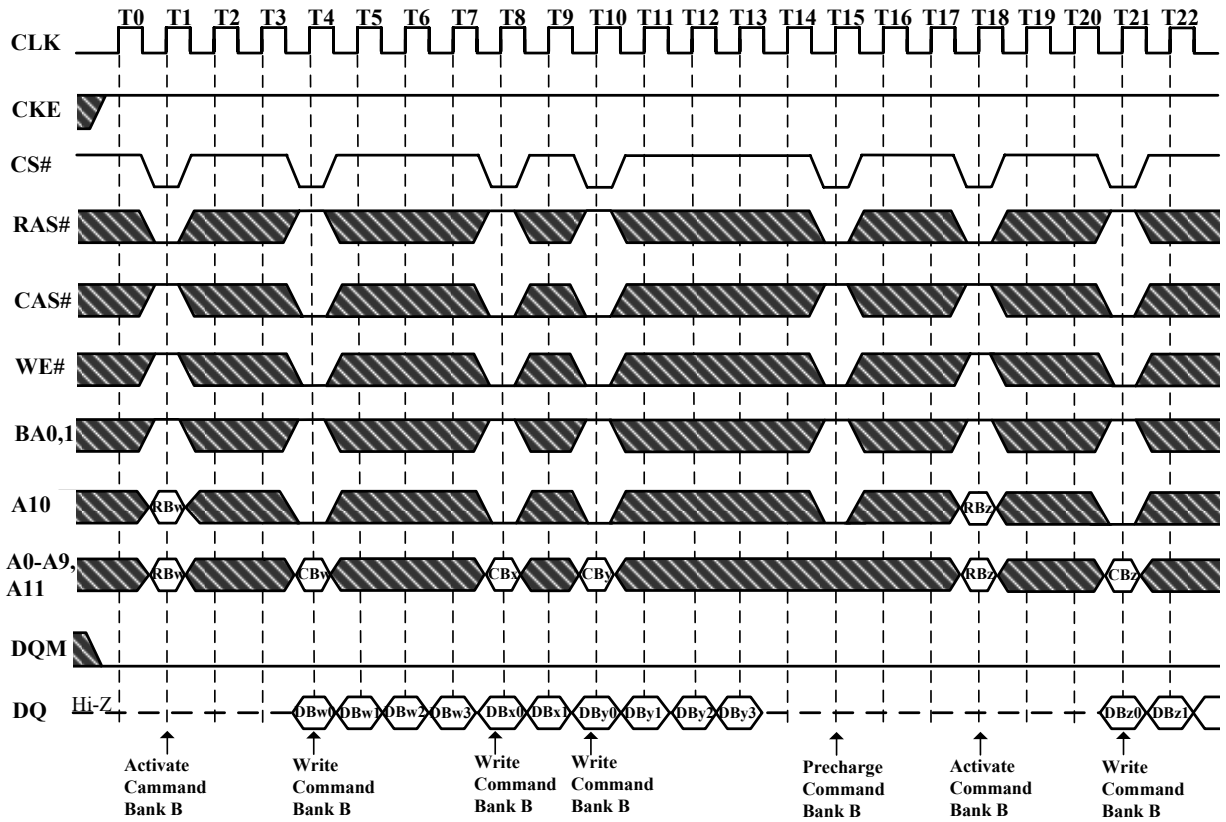
Figure 28. Random Column Write (Page within same Bank) (Burst Length=4)
