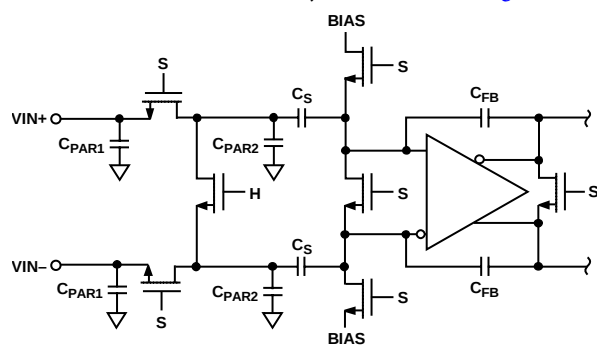
Figure 64. Switched-Capacitor Input
