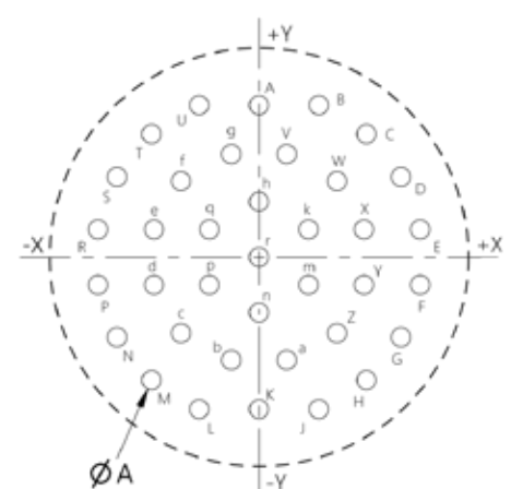
37 Contacts Size 16
