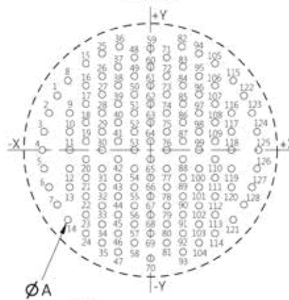
128 Contacts Size 22D
