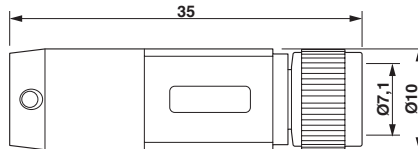
Dimensional drawing
